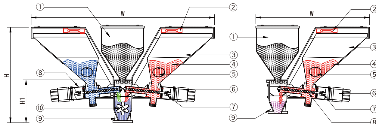
双色称重式色母混合机(带搅拌)工作原理 Working Principle of Dual Color Doser (with Mixing)
